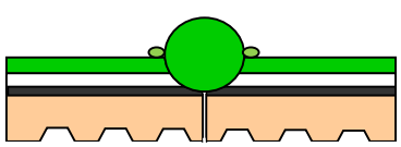
The presence of a small bump indicates the perfect level of fusion of the welding rod.
